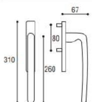
Maniglione singolo \varnothing 10 con conchiglia Single pull handle for sliding door \varnothing 10 with closed plate
