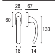
Maniglia per finestra DK \varnothing 7 x 40 Window handle DK \varnothing 7 x 40
